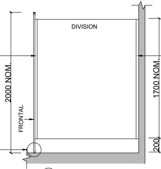
1 SECTION ELEVATION
